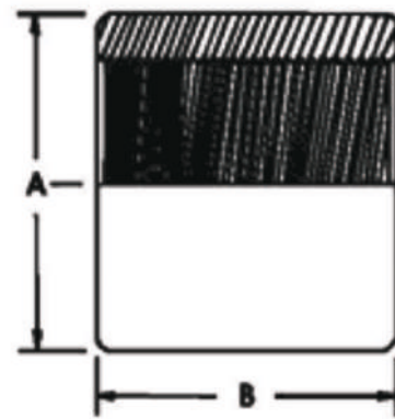
DIMENSIONS OF MILD STEEL SOCKETS
