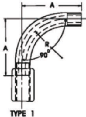
DIMENSIONS OF BENDS
