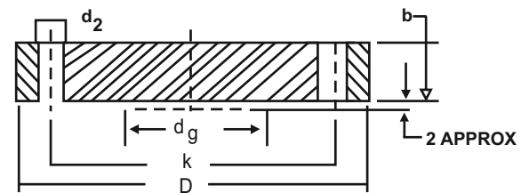
FORM B
