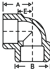
90° ELBOW
