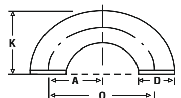
180° SHORT RADIUS ELBOW
