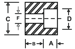
INSERT TYPE 2
