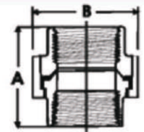
UNION
