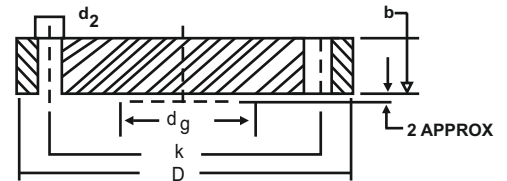
FORM B
