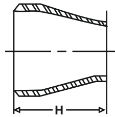
CONCENTRIC REDUCERS
