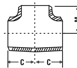
EQUAL TEE
