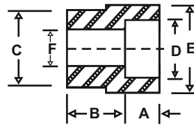
INSERT TYPE 1
